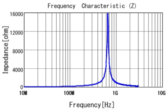
■ LQG15HSR22J02 |Z|
