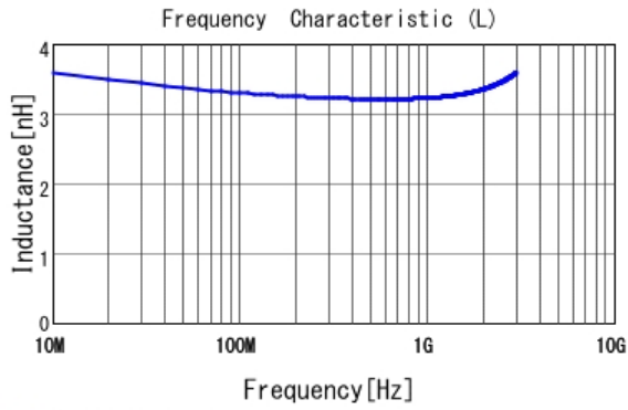
■ LQG15WZ3N3S02 L
