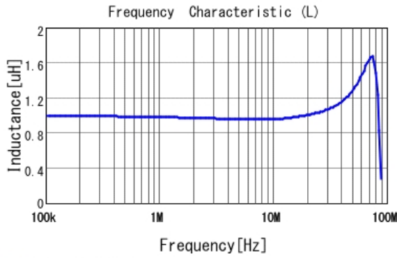
■ LQM21PN1R0MGH L
