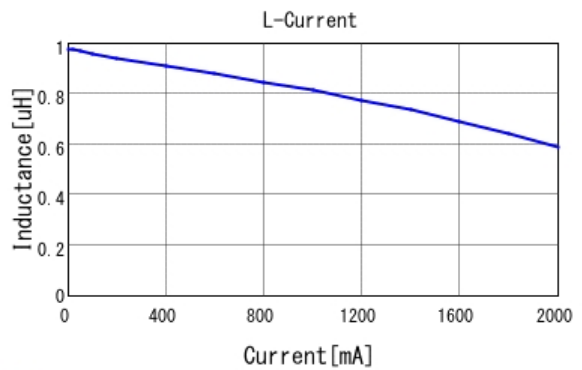
■ LQM21PN1R0MGH L-Current 20degC
