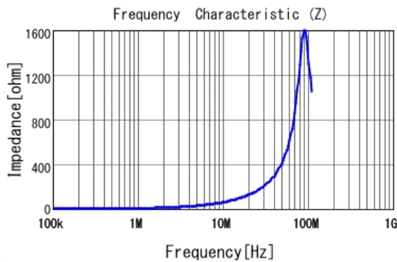
■ LQM21PN1R0MGH |Z|
