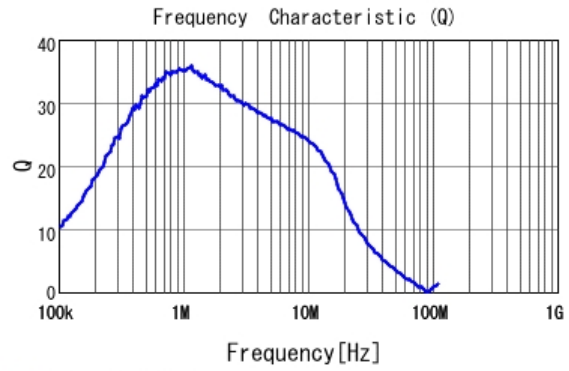
■ LQM21PN1R0MGH Q
