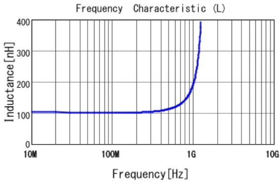
■ LQW2BANR10G00 L
