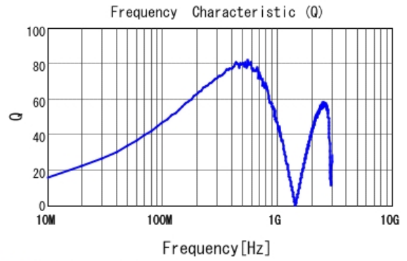
■ LQW2BANR10G00 Q
