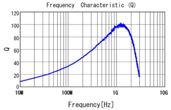
■ LQW2BAS22NJ00 Q
