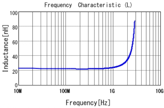
■ LQW2BAS22NJ00 L
