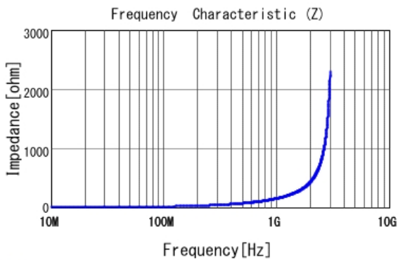
■ LQW2BAS22NJ00 |Z|
