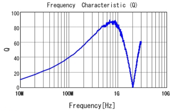
■ LQW2BAS47NJ00 Q
