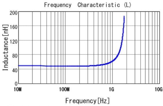
■ LQW2BAS47NJ00 L
