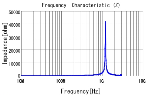
■ LQW2BASR12G00 |Z|
