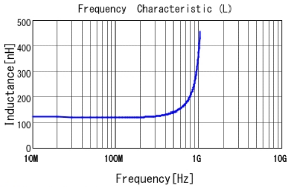
■ LQW2BASR12G00 L
