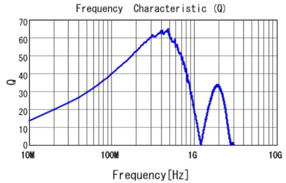
■ LQW2BASR12G00 Q
