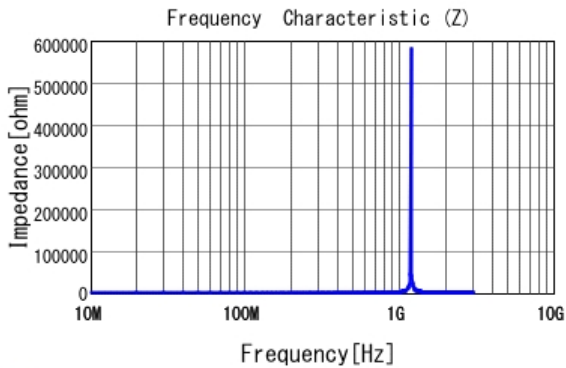
■ LQW2BASR15J00 |Z|
