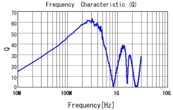
■ LQW2BASR33G00 Q
