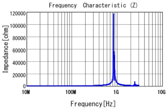
■ LQW2BASR33G00 |Z|
