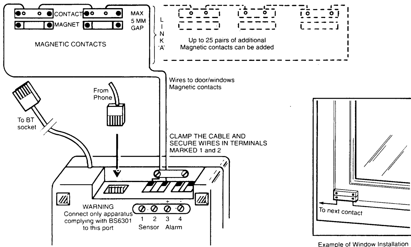
FIGURE 3. Installing the Magnetic Door/Window contacts
