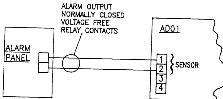
Fig2 ALARM PANEL CONNECTION TO AD01
