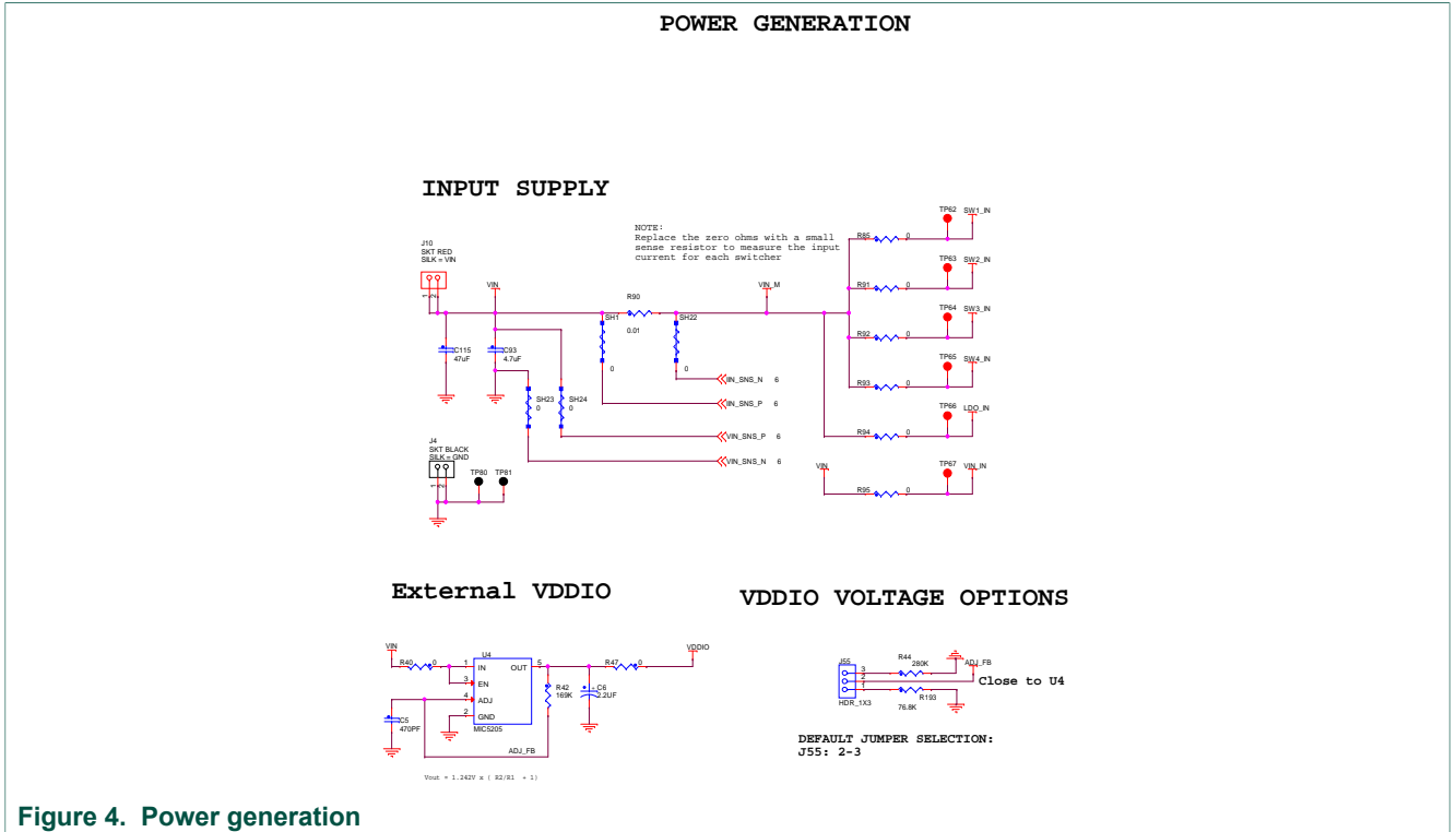
Figure 4. Power generation
