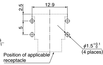
HR12-10R-SP(71) (Stopper plate) (Applicable PCB thickness range 1-2)
