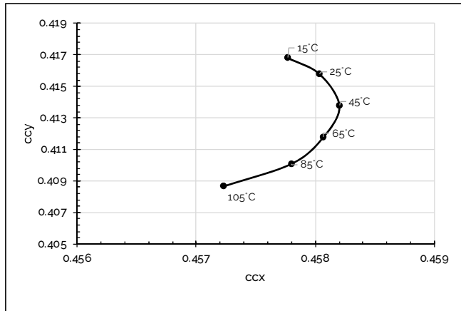
Figure 17: Chromaticity change over Tc, 2700K
