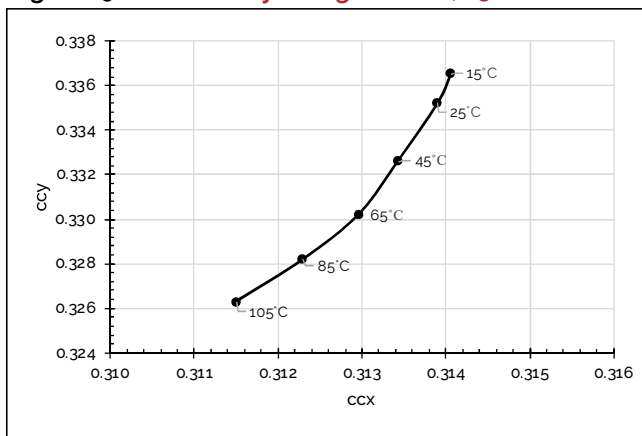
Figure 19: Chromaticity change over Tc, 6500K
