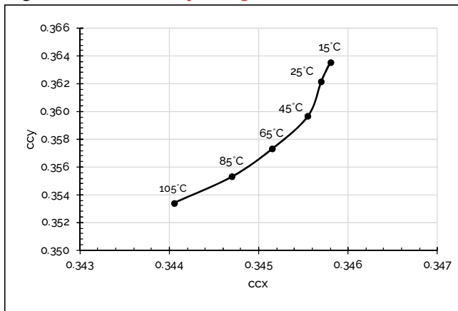
Figure 18: Chromaticity change over Tc, 5000K
