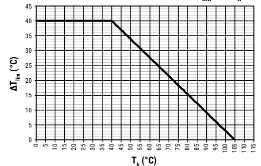
Maximum Overtemperature \Delta T_{lim} vs. T_h
