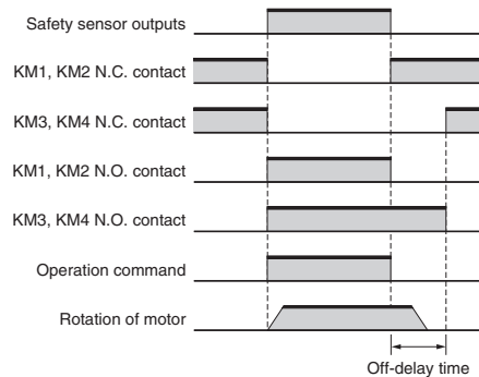
Timing chart
