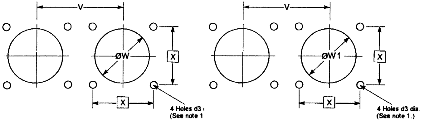
Front Mounting: Style ABCIRH00 ABCIRH04 ABCIRH12A
