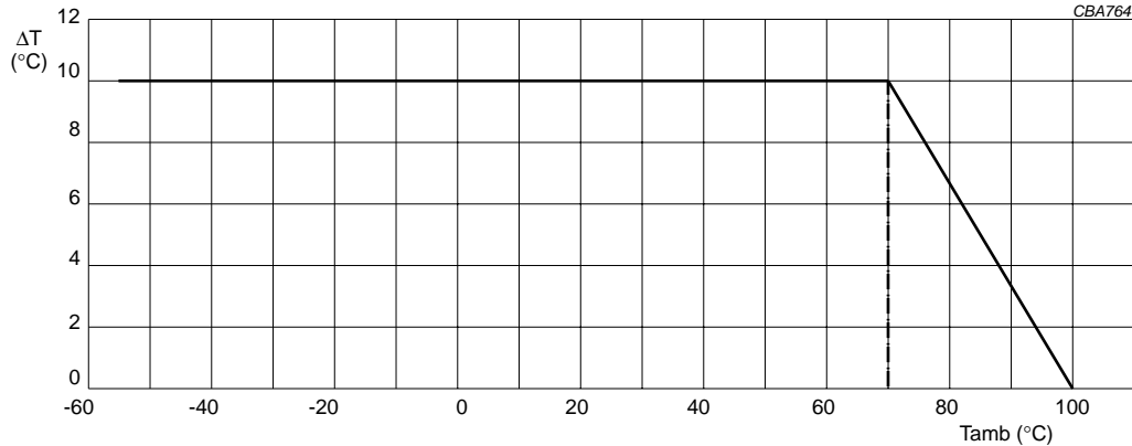
Fig.25 Maximum allowed component temperature rise as a function of the ambient temperature.
