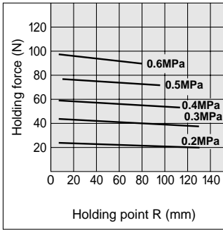
MHL2-32D
