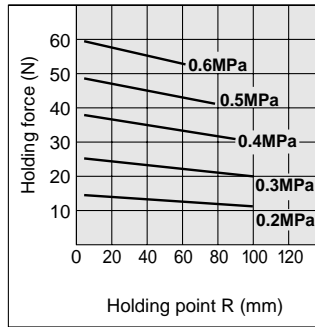
MHL2-25D
