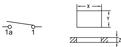
CIRCUIT SPST
