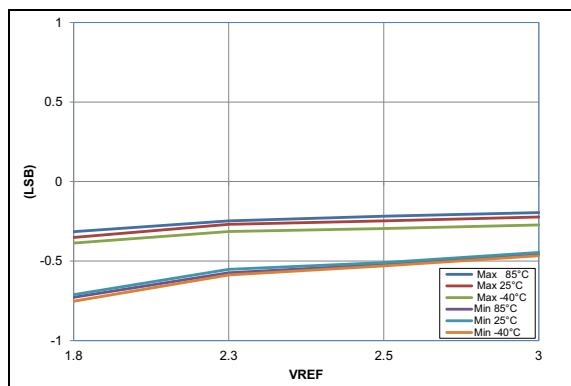
FIGURE 36-66: ADC 10-Bit Mode, Single-Ended Offset Error, V_{DD} = 3.0V , T_{AD} = 4\text{ }\mu\text{s} (All devices)
