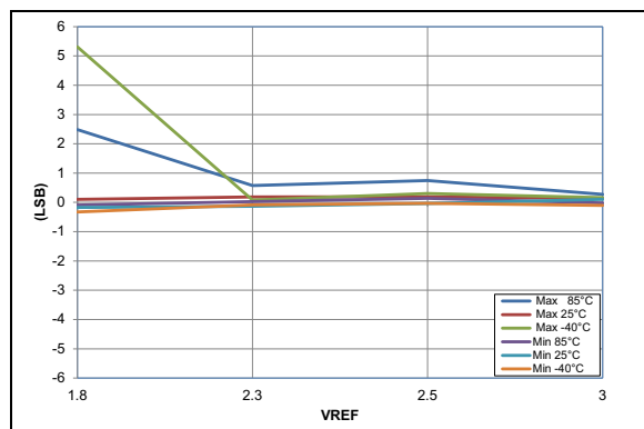
FIGURE 36-65: ADC 10-Bit Mode, Single-Ended Gain Error, V_{DD} = 3.0V , T_{AD} = 4\text{ }\mu\text{s} (All devices)
