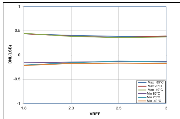
FIGURE 36-63: ADC 10-Bit Mode, Single-Ended DNL, V_{DD} = 3.0V , T_{AD} = 4\text{ }\mu\text{s} (All devices)
