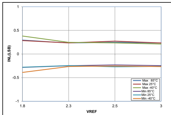
FIGURE 36-64: ADC 10-Bit Mode, Single-Ended INL, V_{DD} = 3.0V , T_{AD} = 4\text{ }\mu\text{s} (All devices)
