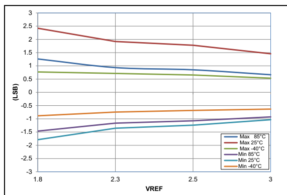
FIGURE 36-62: ADC 10-Bit Mode, Single-Ended Offset Error, V_{DD} = 3.0V , T_{AD} = 1\text{ }\mu\text{s} (All devices)
