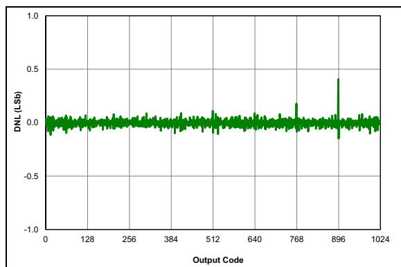
FIGURE 36-53: ADC 10-Bit Mode, Single-Ended DNL, V_{DD} = 3.0V , V_{REF} = 3.0V , T_{AD} = 8\text{ }\mu\text{S} , 25C (All devices)
