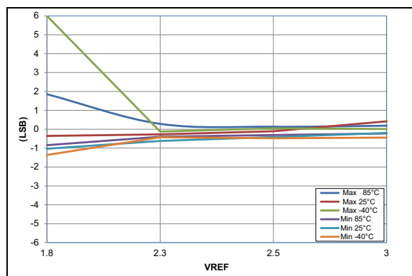
FIGURE 36-61: ADC 10-Bit Mode, Single-Ended Gain Error, V_{DD} = 3.0V , T_{AD} = 1\text{ }\mu\text{s} (All devices)
