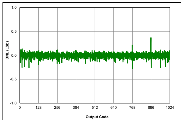
FIGURE 36-51: ADC 10-Bit Mode, Single-Ended DNL, V_{DD} = 3.0V , V_{REF} = 3.0V , T_{AD} = 1\text{ }\mu\text{S} , 25C (All devices)
