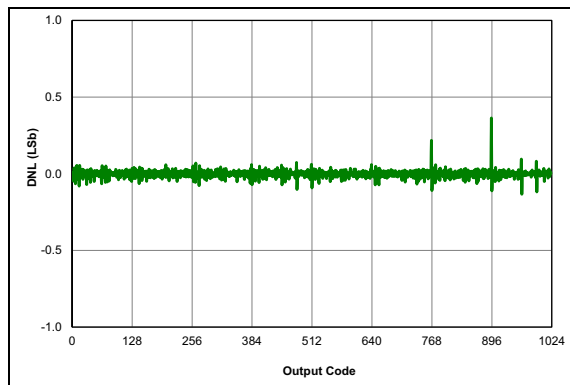
FIGURE 36-52: ADC 10-Bit Mode, Single-Ended DNL, V_{DD} = 3.0V , V_{REF} = 3.0V , T_{AD} = 4\text{ }\mu\text{S} , 25C (All devices)
