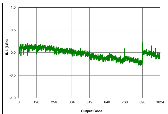
FIGURE 36-54: ADC 10-Bit Mode, Single-Ended INL, V_{DD} = 3.0V , V_{REF} = 3.0V , T_{AD} = 1\text{ }\mu\text{S} , 25C (All devices)
