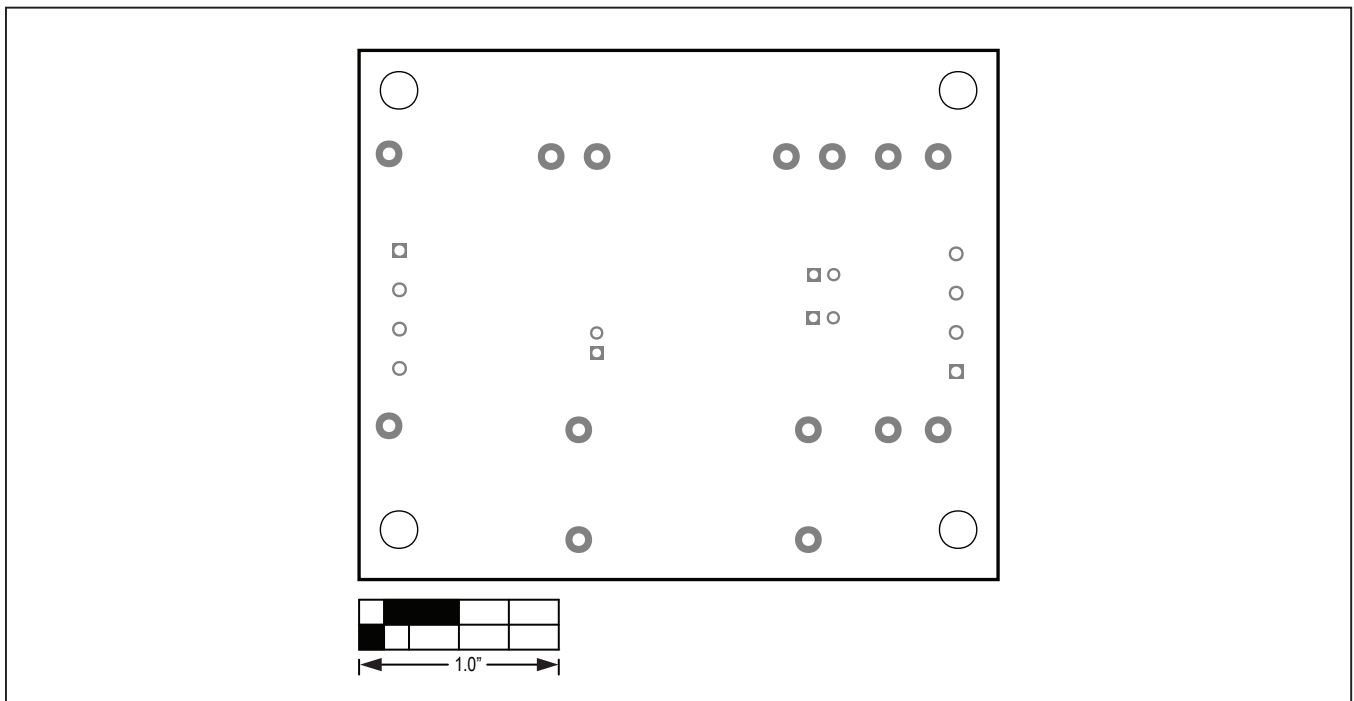
MAX22518 EV Kit Component Placement Guide—Bottom Silkscreen
