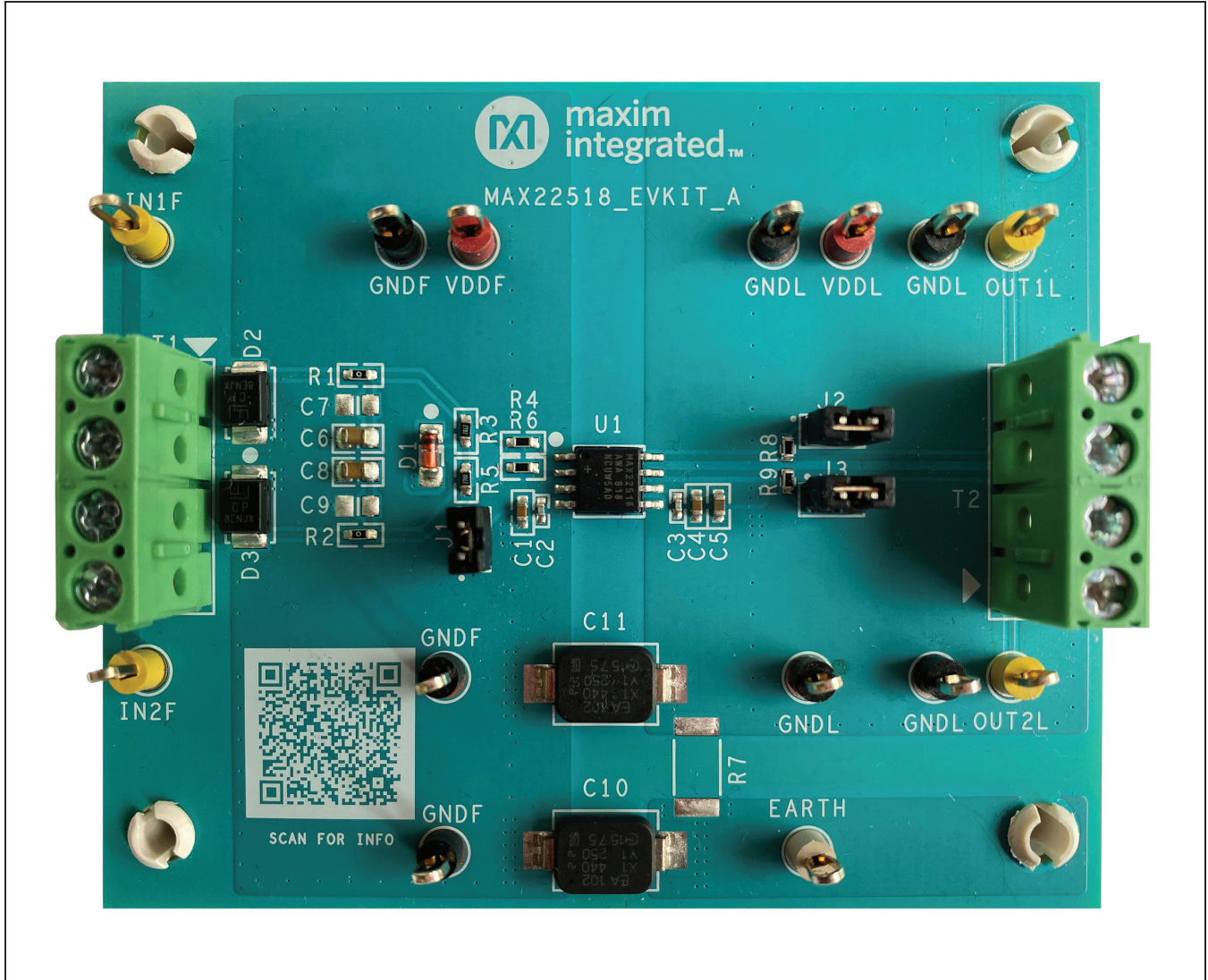
Figure 1. MAX22518EVKIT#
