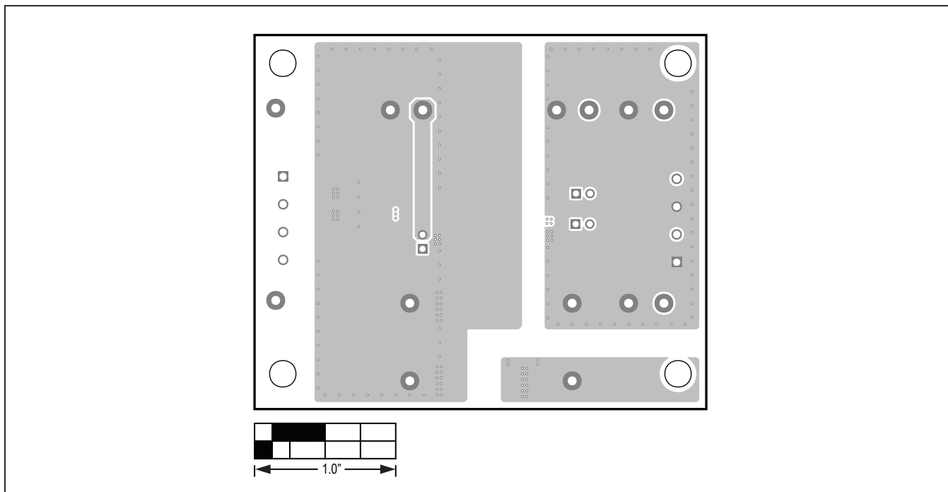
MAX22518 EV Kit PCB Layout—L2 GND
