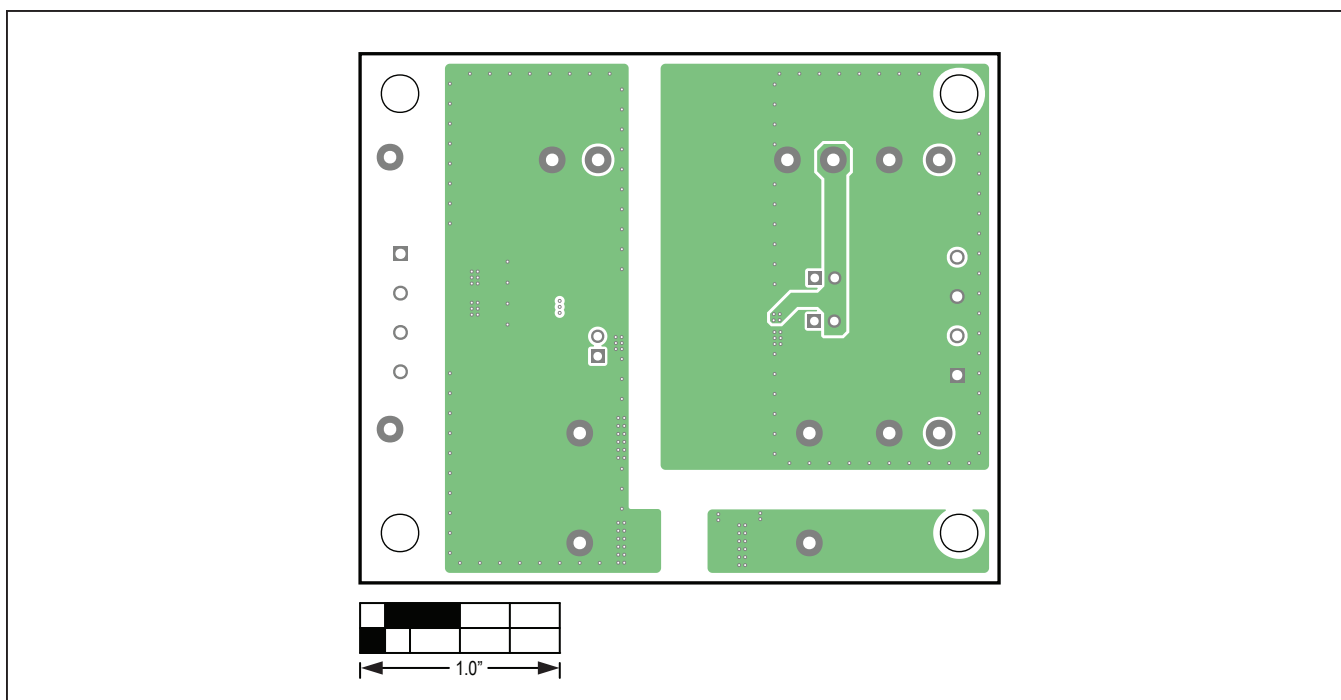
MAX22518 EV Kit PCB Layout—L3 GND
