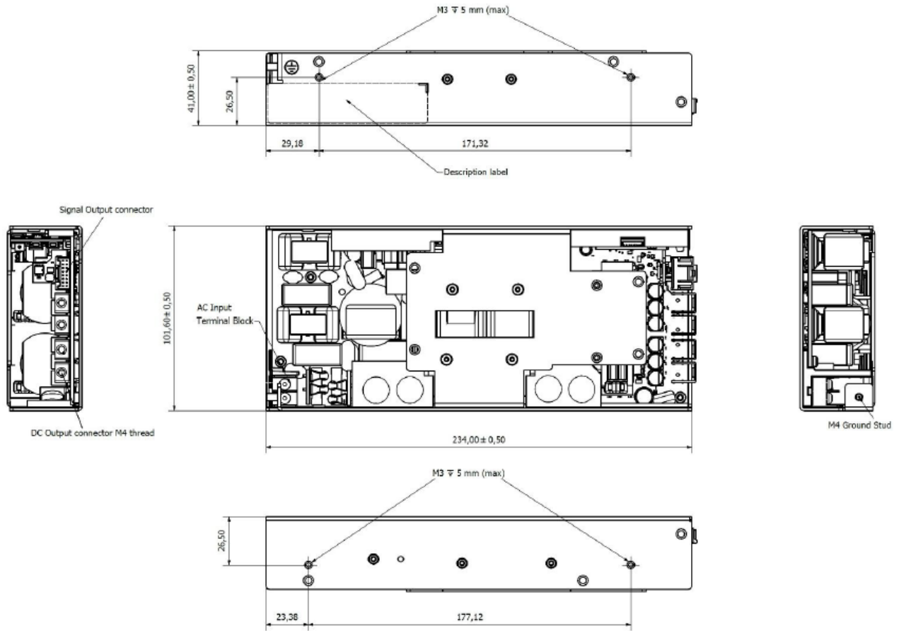
Figure 2. Mechanical Drawing – MCC750-1T24 / MCC750-1T48 Models
