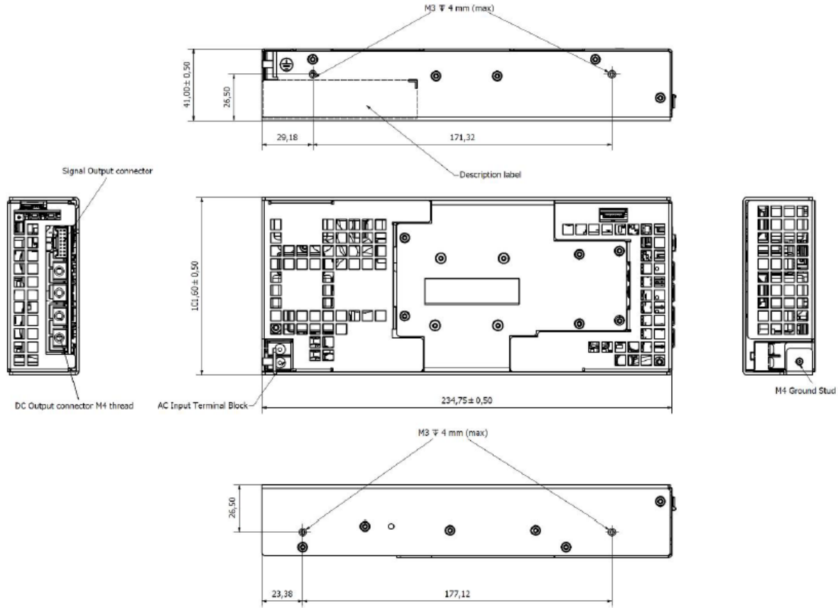
Figure 5. Mechanical Drawing - MCC750-1T24-PC / MCC750-1T48-PC Models
