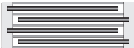
Extended double side metallized carrier film design
