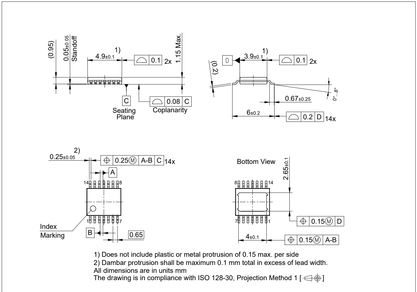
Figure 10 PG-TSDSO-14
