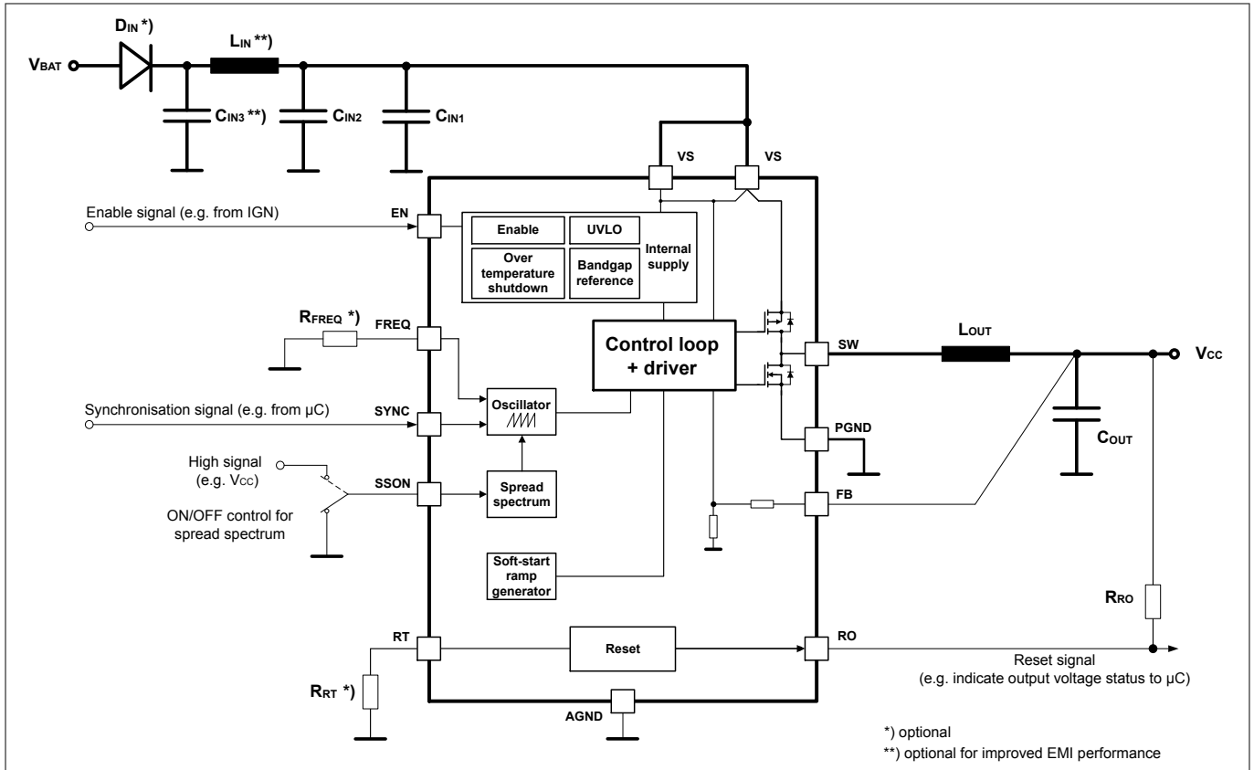
Figure 9 Application diagram
