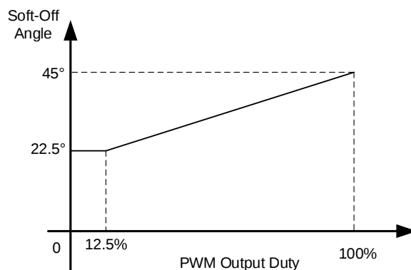
Figure 4: Soft-Off Angle vs. Output Duty
