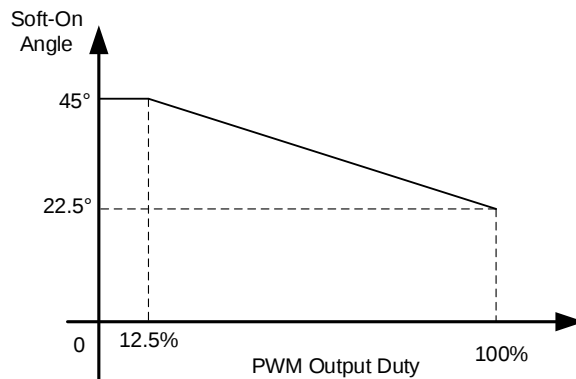
Figure 3: Soft-On Angle vs. Output Duty
