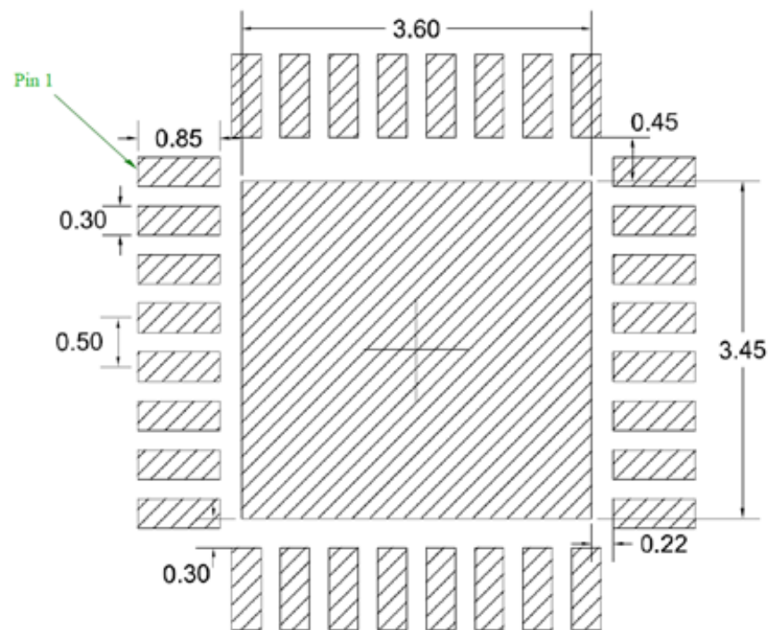
Figure 33. VFQFPN (5X5X0.95) 32L recommended footprint
