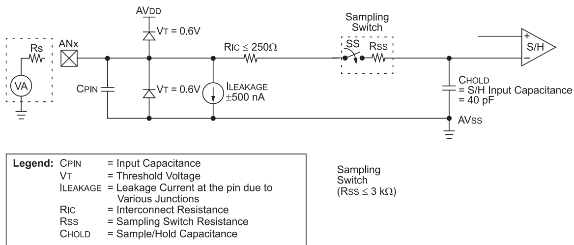
Figure 22-3. 12-Bit A/D Converter Analog Input Model
