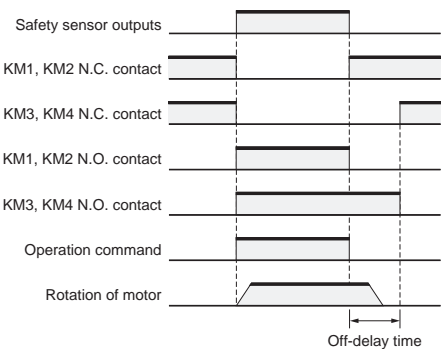
Timing chart
