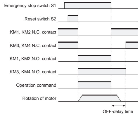
Timing chart
