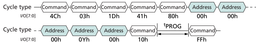
Figure 65: Address and Command Cycles
