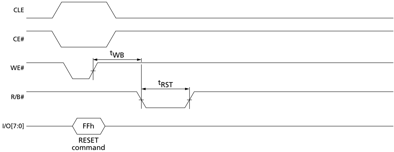
Figure 81: RESET Operation
