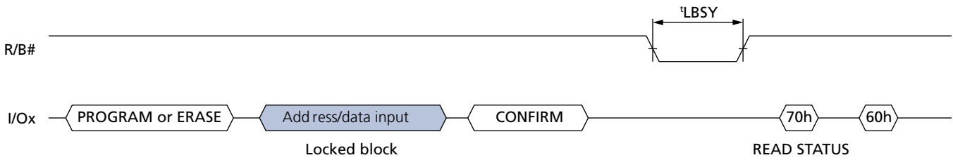
Figure 23: PROGRAM/ERASE Issued to Locked Block
