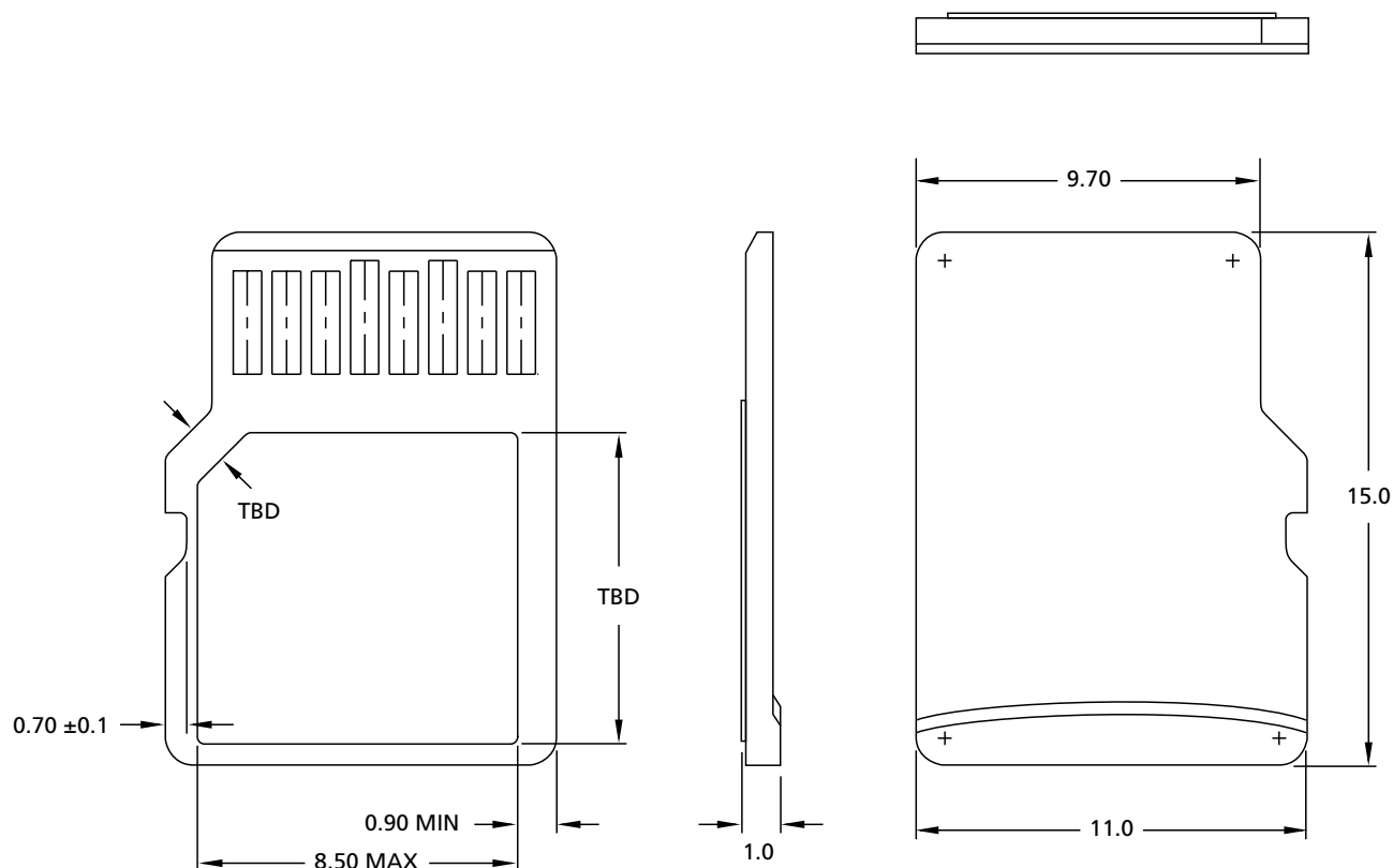
Figure 4: microSD Card – 11mm x 15mm
