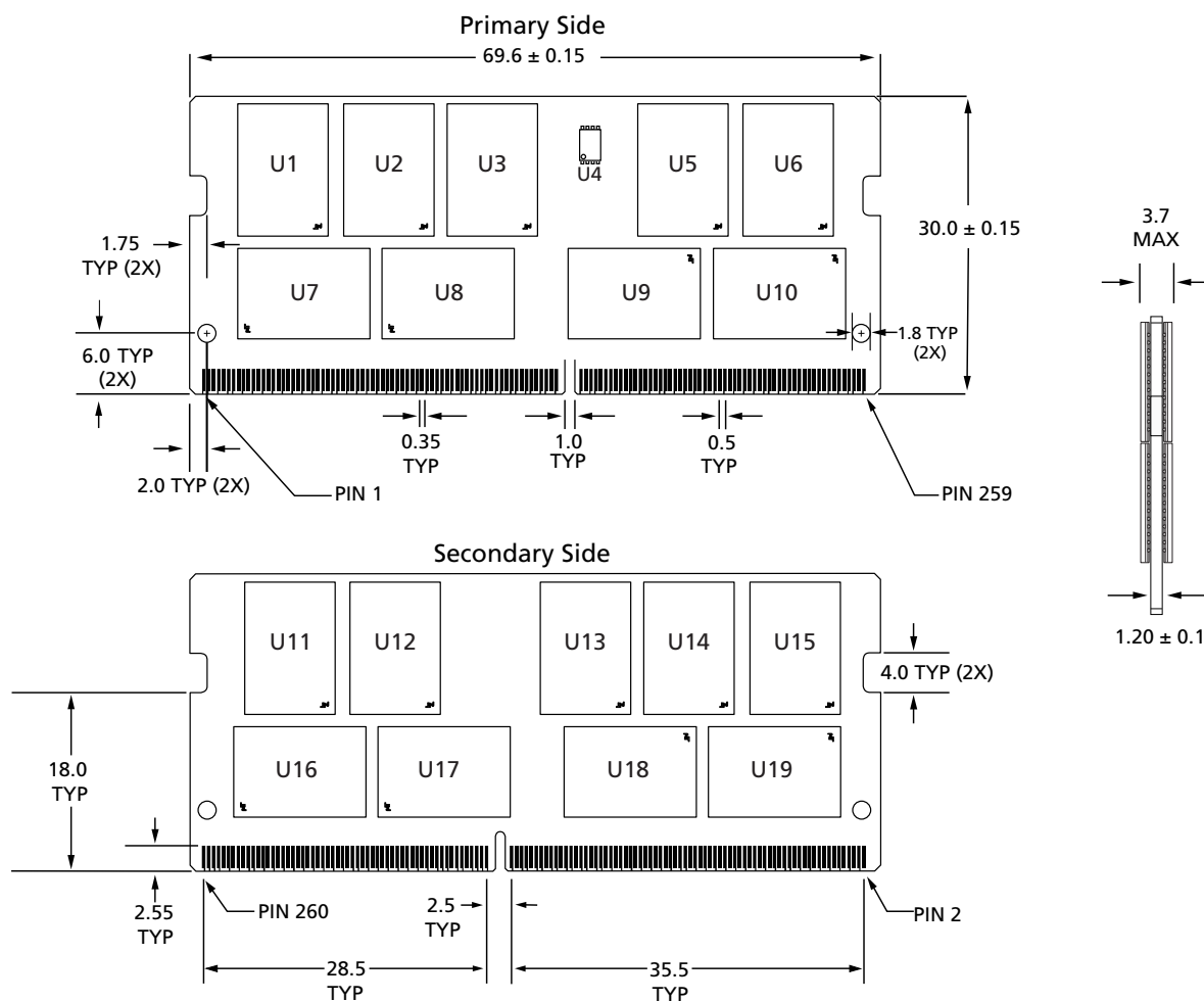
Figure 5: 260-Pin DDR4 SODIMM, R/C-H (PCB 1813)
