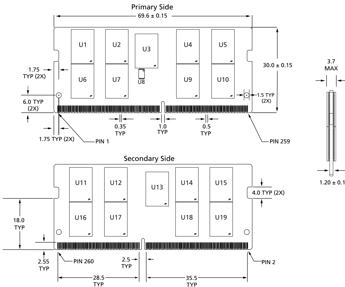
Figure 6: 260-Pin DDR4 SODIMM, R/C-G1 (PCB 2451)
