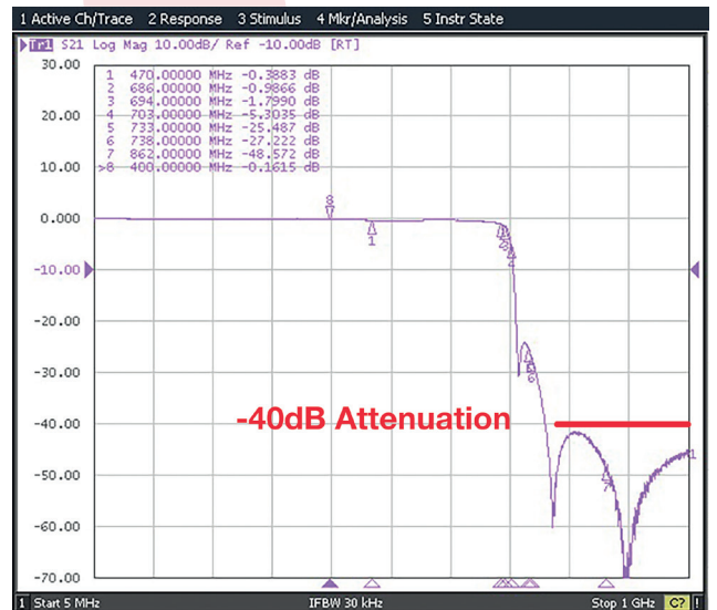
F5GO Masthead Outdoor 4G-5G Filter with F Connections
