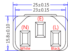
ME-302 (IEC 60320, C13, 13A 125V~) (Dimensions of Connector Face)
