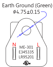
ME-301 (NEMA 5-15P) (Dimensions of Plug Face)
