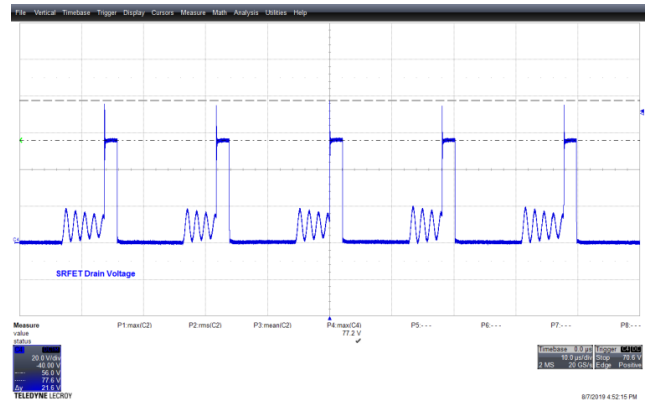
Figure 142 – 265 VAC 50 Hz, V_{USB-C} = 9\text{ V} Full Normal. V_{DRAIN} , 20 V / div., 10 \mu\text{s} / div. V_{DS} = 77.2\text{ V} .
