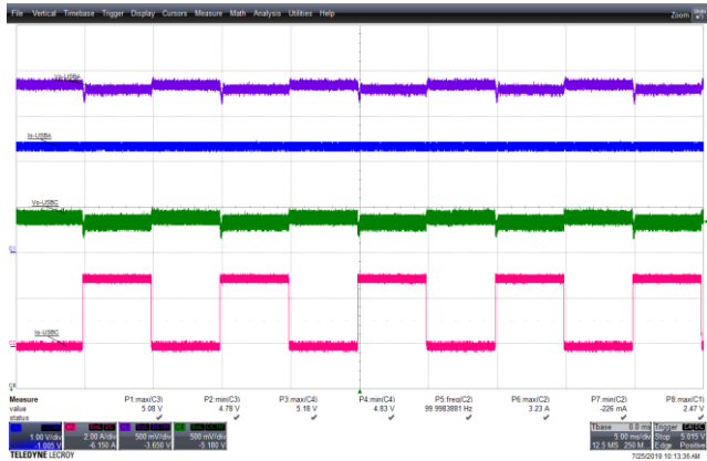
Figure 93 – 90 VAC 60 Hz, 0-3 A USB-C Transient Load CH1(Blue): I_{USB-A} , 1 A / div., 5 ms / div. CH2(Pink): I_{USB-C} , 2 A / div. CH3(Violet): V_{USB-A} , 0.5 V / div. CH4(Green): V_{USB-C} , 0.5 V / div.
