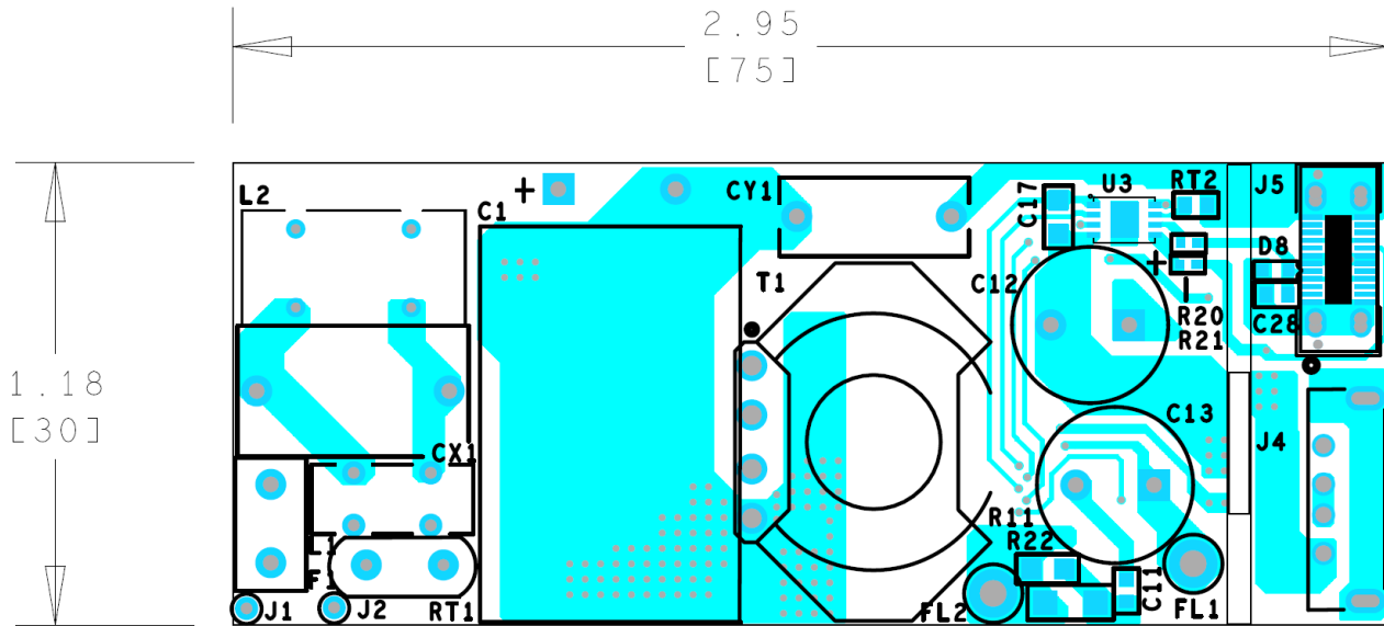
Figure 8 – Top Side.
