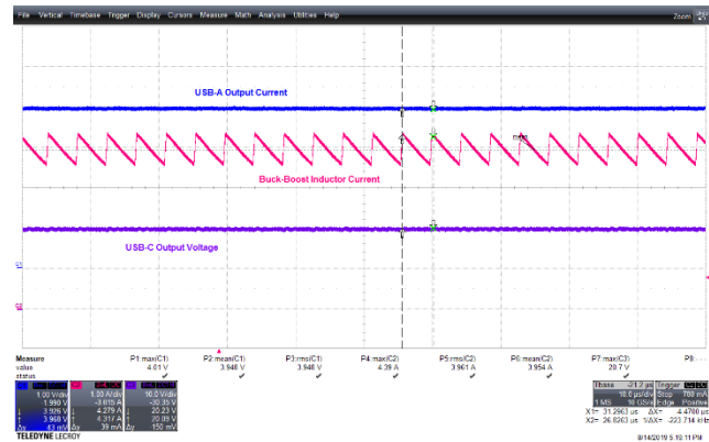
Figure 128 – 265 VAC 60 Hz, USB-A Full Load Short. CH1(Blue): I_{USB-A} , 1 A / div., 10 \mu\text{s} / div. CH2(Pink): I_{L3} , 1 A / div. CH3(Violet): V_{USB-C} , 10 V / div.
