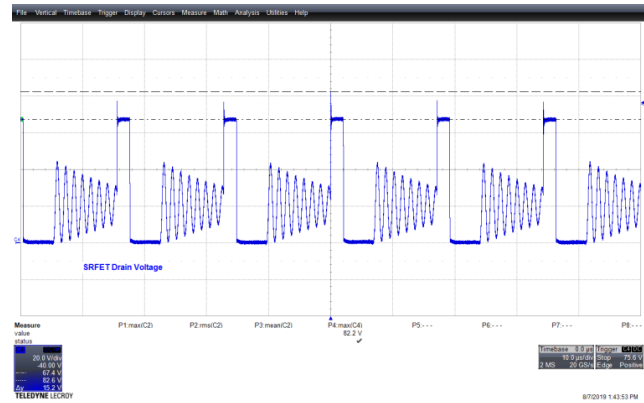
Figure 136 – 265 VAC 50 Hz, V_{USB-C} = 20 V Full Normal. V_{DRAIN} , 20 V / div., 10 \mu s / div. V_{DS} = 82.2 V.
