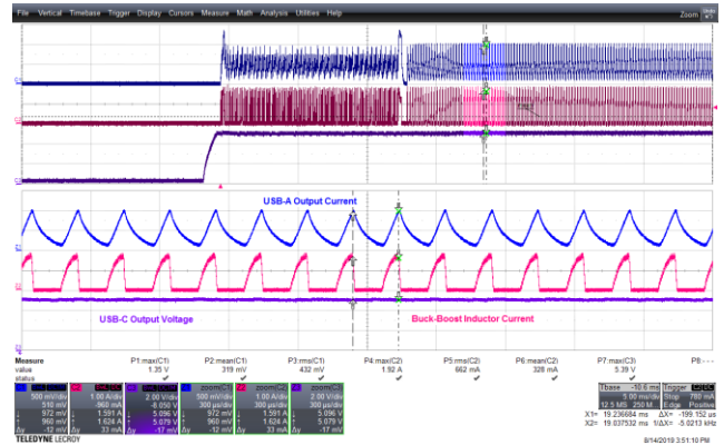
Figure 124 – 265 VAC 60 Hz, USB-A Start-up Short. CH1(Blue): I_{USB-A} , 0.5 A / div., 5 ms / div. CH2(Pink): I_{L3} , 1 A / div. CH3(Violet): V_{USB-C} , 2 V / div.
