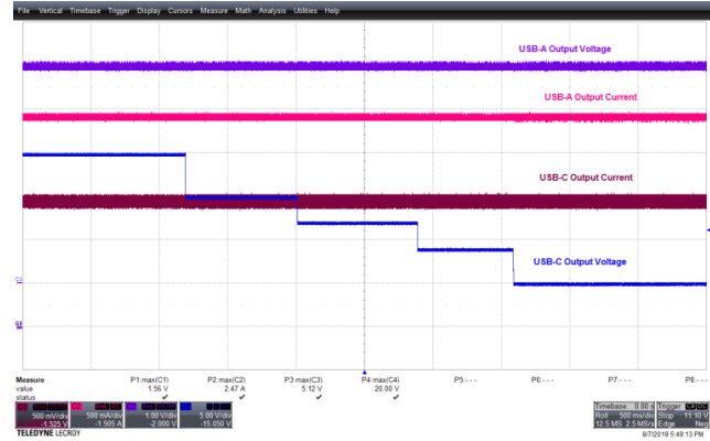
Figure 88 – 265 VAC 60 Hz, 20 V - 15 V - 12 V - 9 V - 5 V.
