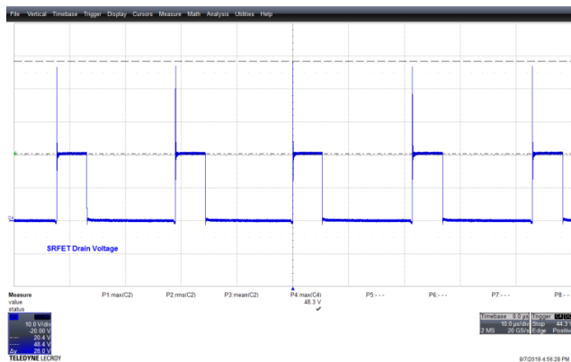
Figure 143 – 90 VAC 60 Hz, V_{USB-C} = 9\text{ V} Full Normal. V_{DRAIN} , 20 V / div., 10 \mu\text{s} / div. V_{DS} = 48.3\text{ V} .
