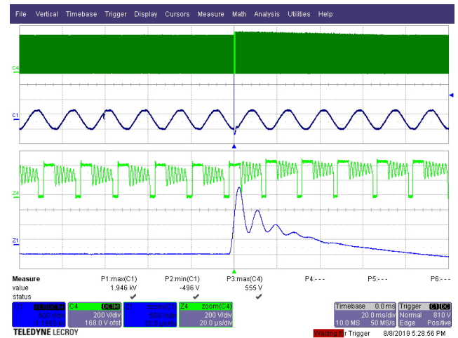
Figure 163 – 230 VAC 50 Hz, 2 kV Differential Surge
