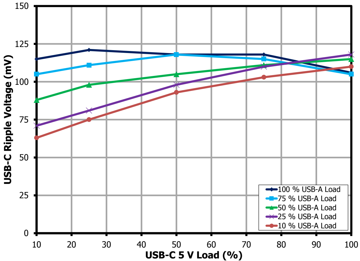
Figure 33 – USB-C Ripple Voltage vs. USB-A / USB-C Load @ 90 VAC.
