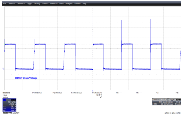
Figure 141 – 90 VAC 60 Hz, V_{USB-C} = 9\text{ V} Full Normal. V_{DRAIN} , 20 V / div., 10 \mu\text{s} / div. V_{DS} = 52.8\text{ V} .
