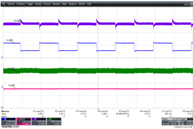
Figure 103 – 90 VAC 60 Hz, 1.2-2.4 A USB-A Transient. CH1(Blue): I_{USB-Ar} 2 A / div., 5 ms / div. CH2(Pink): I_{USB-Cr} 2 A / div. CH3(Violet): V_{USB-A} 1 V / div. CH4(Green): V_{USB-C} 0.5 V / div.
