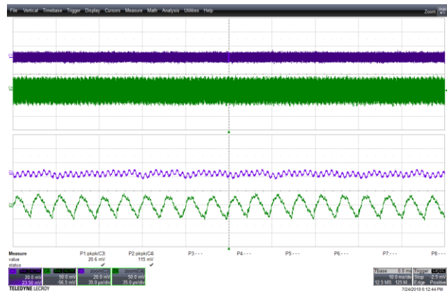
Figure 112 – 265 VAC 50 Hz, Full Load Normal. Upper: V_{USB-A} , 50 mV / div., 10 ms / div. Lower: V_{USB-C} , 50 mV / div. V_{RIPPLE(USB-A)} = 20.6\text{ mVpp} . V_{RIPPLE(USB-C)} = 115\text{ mVpp} .
