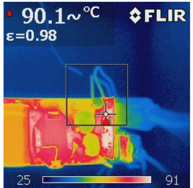
Figure 49 – Buck-boost Inductor (L23): 90.1 °C.
