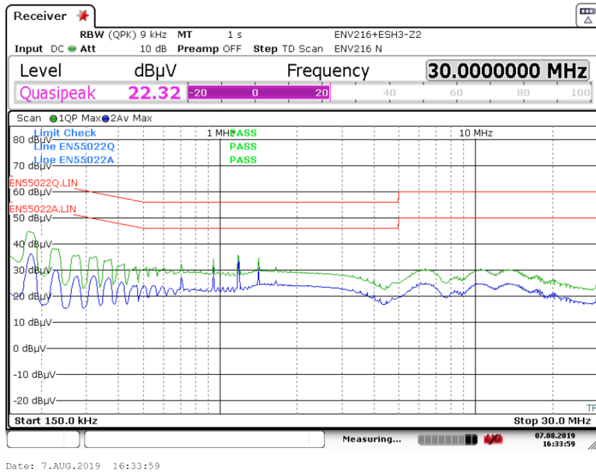
Figure 155 – Conducted EMI at V_{USB-C}=5 V Full Load, 115 VAC 60 Hz Line N.
