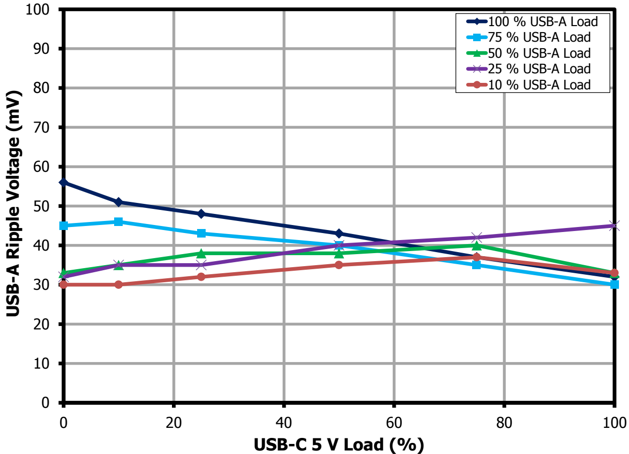
Figure 37 – USB-A Ripple Voltage vs. USB-A / USB-C Load @ 90 VAC.
