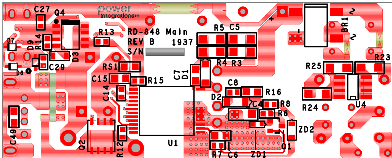
Figure 9 – Bottom Side.
