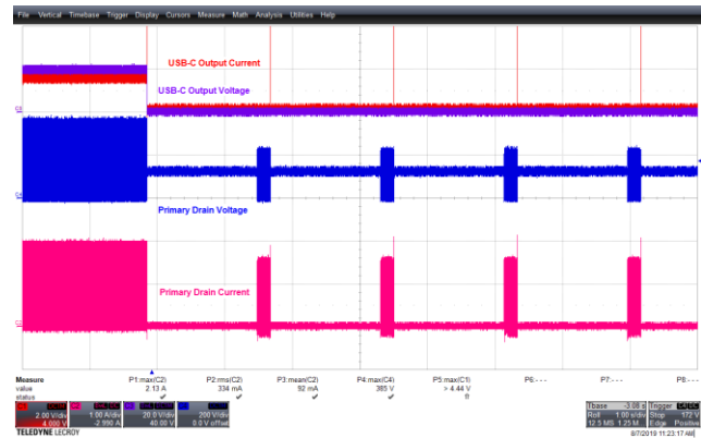
Figure 120 – 265 VAC 50 Hz, USB-C Full Load Short. CH1(Red): I_{USB-C} , 2 A / div., 1 s / div. CH2(Pink): I_{DRAIN} , 1 A / div. CH3(Violet): V_{USB-C} , 20 V / div. CH4(Blue): V_{DRAIN} , 200 V / div.
