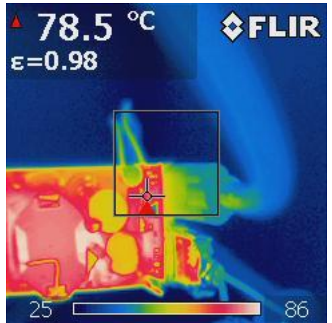
Figure 65 – Buck-boost Inductor (L23): 78.5 °C.
