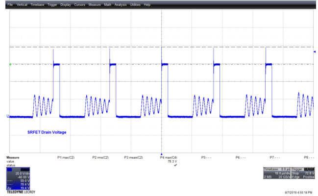
Figure 140 – 265 VAC 50 Hz, V_{USB-C} = 12\text{ V} Full Normal. V_{DRAIN} , 20 V / div., 10 \mu\text{s} / div. V_{DS} = 78.3\text{ V} .
