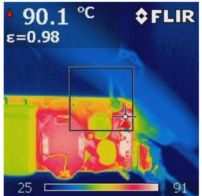
Figure 57 – Buck-boost Inductor (L3): 90.1 °C.
