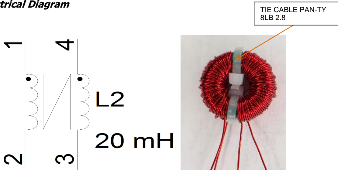
Figure 16 – Inductor Electrical Diagram.
