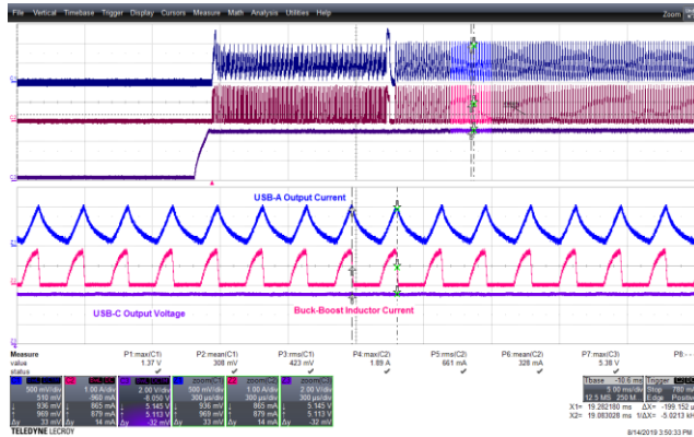
Figure 123 – 90 VAC 60 Hz, USB-A Start-up Short. CH1(Blue): I_{USB-A} , 0.5 A / div., 5 ms / div. CH2(Pink): I_{L3} , 1 A / div. CH3(Violet): V_{USB-C} , 2 V / div.
