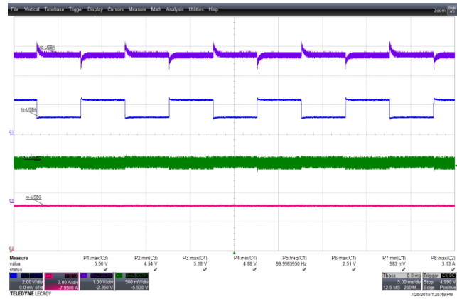
Figure 104 – 265 VAC 50 Hz, 1.2-2.4 A USB-A Transient. CH1(Blue): I_{USB-Ar} 2 V / div., 5 ms / div. CH2(Pink): I_{USB-Cr} 2 A / div. CH3(Violet): V_{USB-A} 1 V / div. CH4(Green): V_{USB-C} 0.5 V / div.
