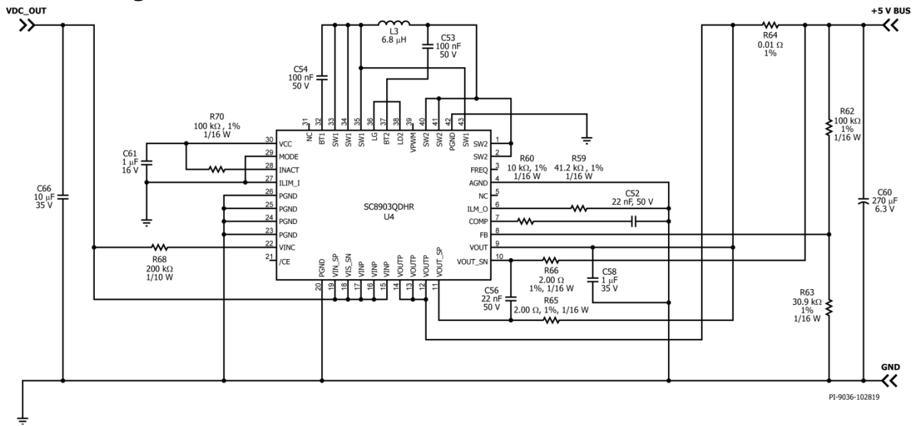
Figure 7 – Daughter Board Schematic.
