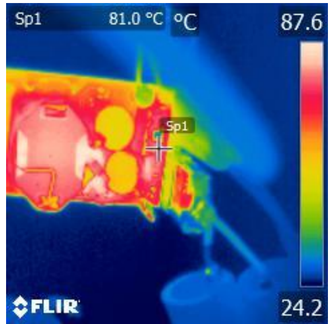
Figure 73 – Buck-boost Inductor (L3): 81 °C.
