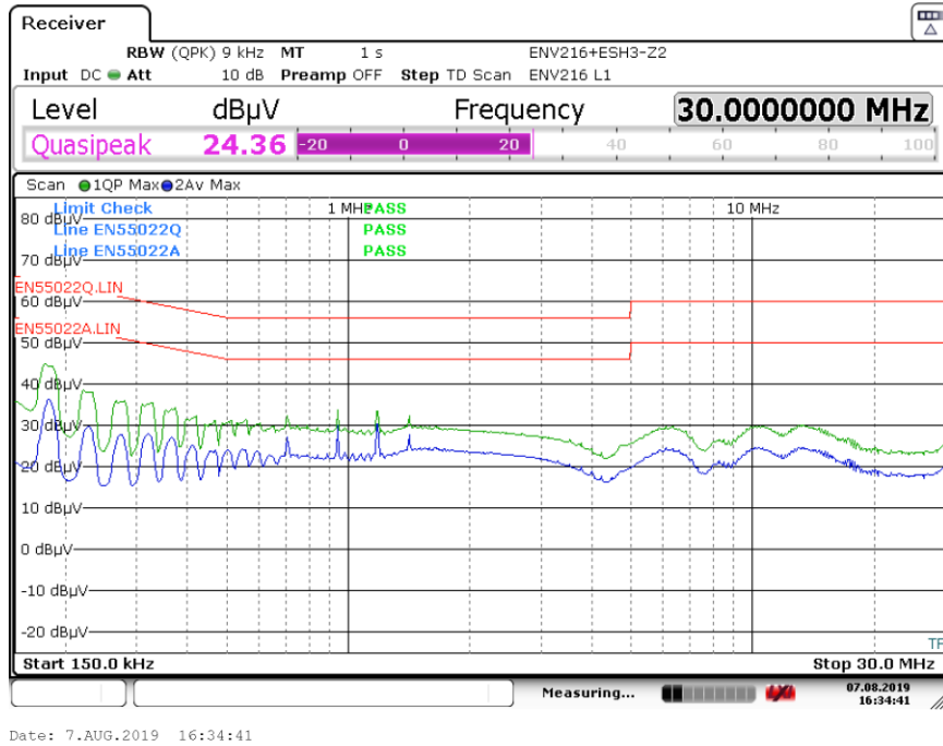
Figure 154 – Conducted EMI at V_{USB-C}=5 V Full Load, 115 VAC 60 Hz Line L.
