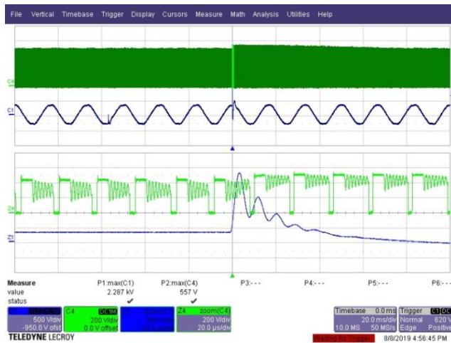
Figure 162 – 230 VAC 50 Hz, 2 kV Differential Surge
