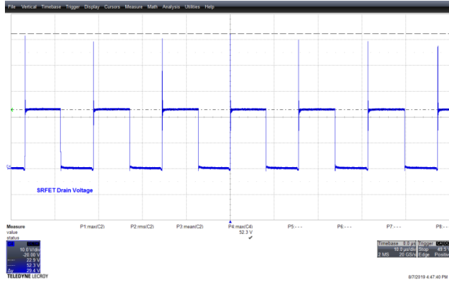
Figure 139 – 90 VAC 60 Hz, V_{USB-C} = 12\text{ V} Full Normal. V_{DRAIN} , 20 V / div., 10 \mu\text{s} / div. V_{DS} = 52.3\text{ V} .
