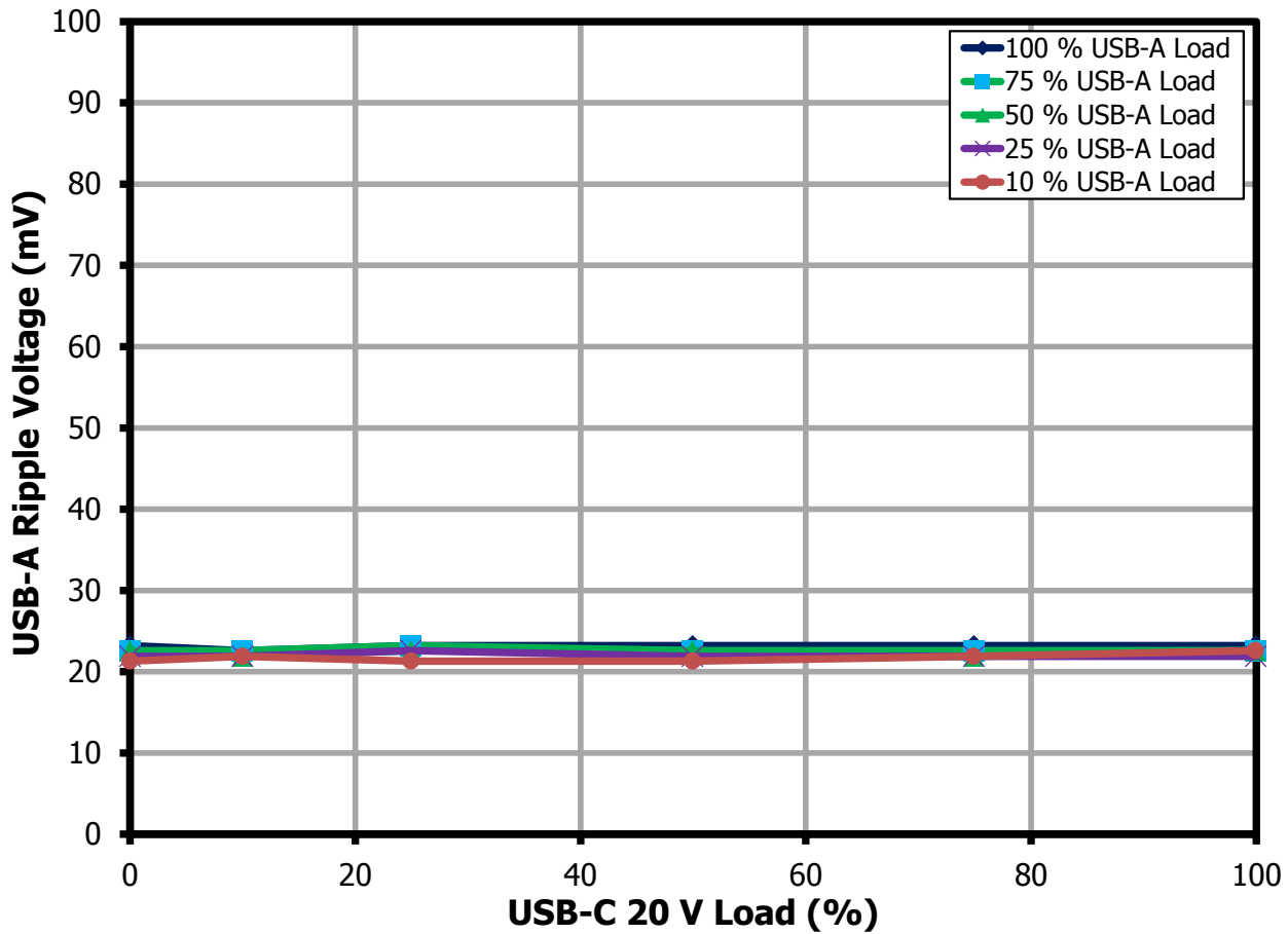
Figure 39 – USB-A Ripple Voltage vs. USB-A / USB-C Load @ 90 VAC.
