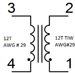
Figure 14 – Inductor Electrical Diagram.
