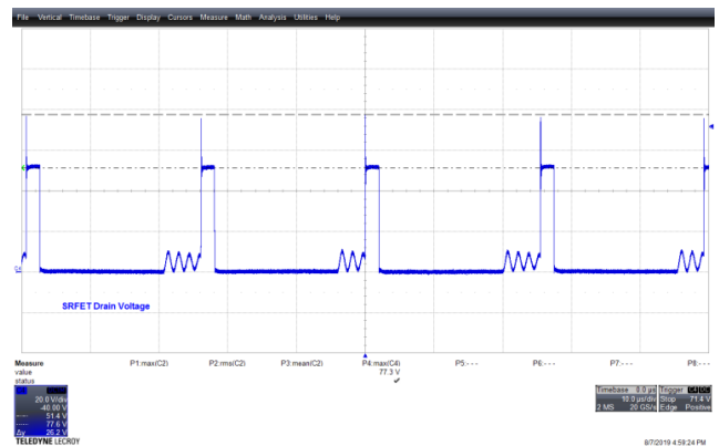
Figure 144 – 265 VAC 50 Hz, V_{USB-C} = 9\text{ V} Full Normal. V_{DRAIN} , 20 V / div., 10 \mu\text{s} / div. V_{DS} = 77.3\text{ V} .
