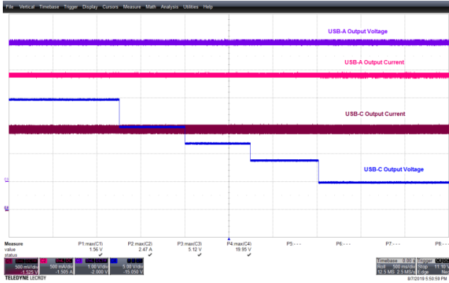
Figure 87 – 90 VAC 60 Hz, 20 V - 15 V - 12 V - 9 V - 5 V.
