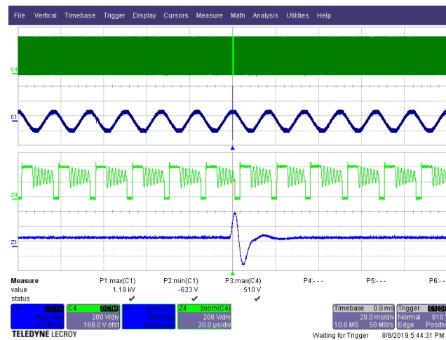
Figure 165 – 230 VAC 50 Hz, 2.5kV Ring Wave L/N. Injection Phase: 270° Upper: V DRAIN , 200 V / div. Lower: V IN , 500 V / div., 20 ms / div. VDS = 510 V.
