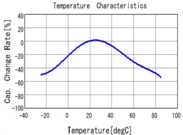
■ DE2E3SA222MN3AX02F C-Temp. capchange, DCOV, AC1Vrms
