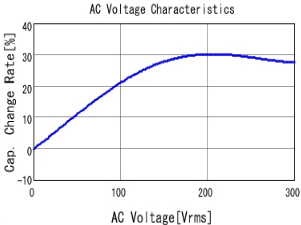
■ DE2E3SA222MN3AX02F C-AC Voltage capchange, DCOV, 20.0
