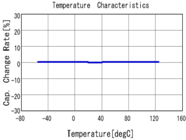
■ GCM1555C1H7R0CA16 C-Temp. capchange, DCOV, AC1Vrms
