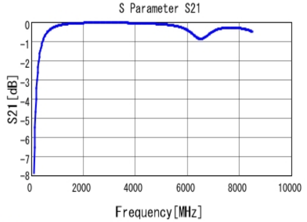
■ GCM1555C1H7R0CA16 S21 DCOV, 25degC
