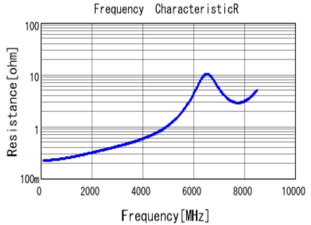
■ GCM1555C1H7R0CA16 R DC0V, 25degC
