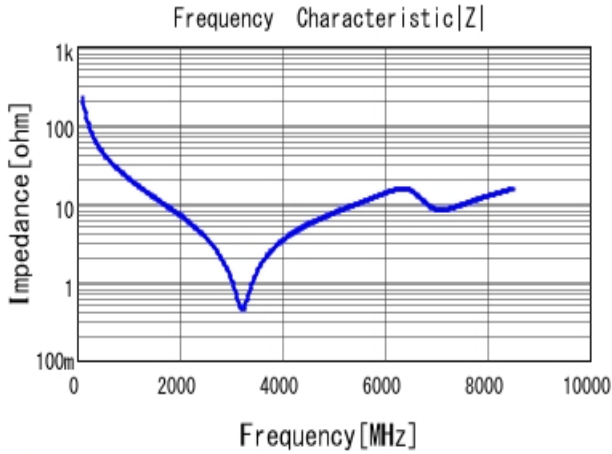
■ GCM1555C1H7R0CA16 |Z| DC0V, 25degC
