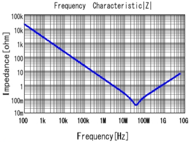
■ GRM033C81A104KE14 |Z| DCOV, 25degC
