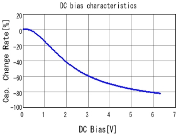
■ GRM155B30J475ME87 C-DC bias capchange, 20.0degC, AC0.
