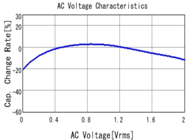
■ GRM155B30J475ME87 C-AC Voltage capchange, DCOV, 20.0d
