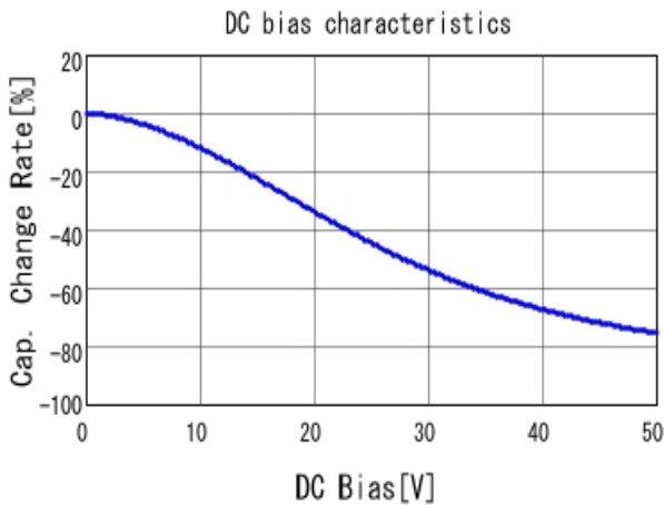
■ KRM31KR71H475KH01 C-DC bias capchange, 25.0degC, AC1V
