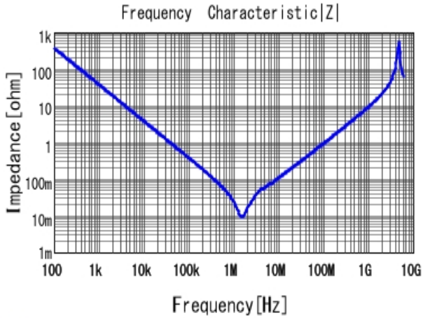
■ KRM31KR71H475KH01 |Z| DCOV, 25degC
