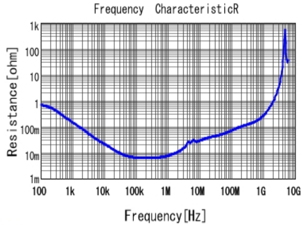
■ KRM31KR71H475KH01 R DCOV, 25degC
