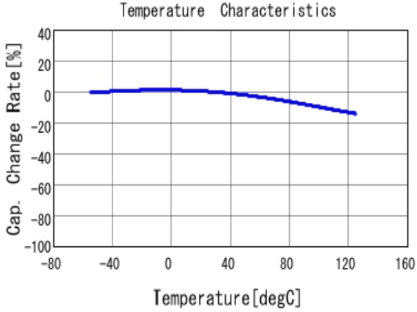
■ KRM31KR71H475KH01 C-Temp. capchange, DCOV, AC1Vrms
