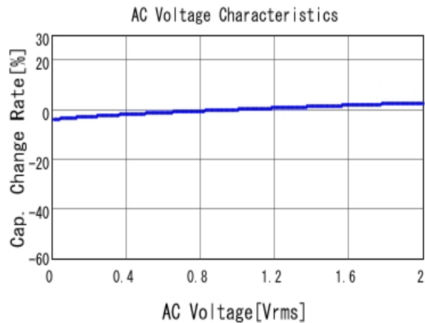
■ KRM31KR71H475KH01 C-AC Voltage capchange, DCOV, 25.0d
