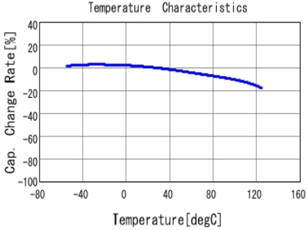
■ GCJ32EC71H106KA01 C-Temp. capchange, DC0.0V, AC1.0V rm
