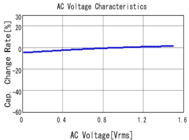
■ GCJ32EC71H106KA01 C-AC Voltage capchange, DCOV, 25.0d
