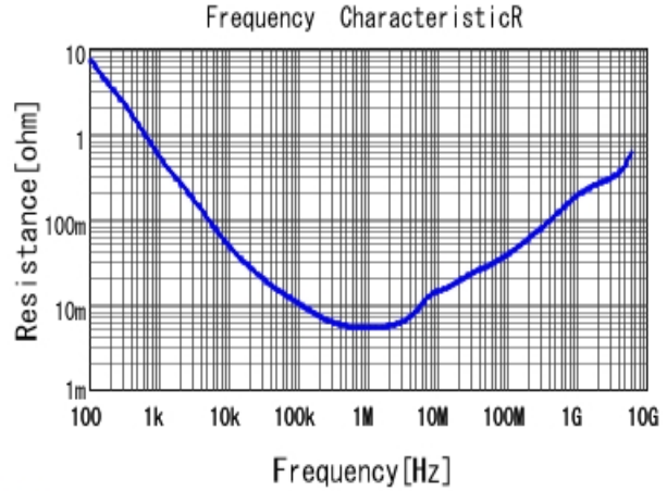
■ GRM155B30J475ME47 R DCOV, 20degC
