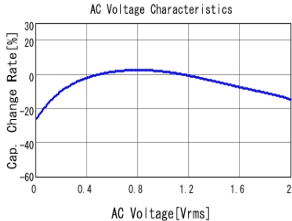
■ GRM155B30J475ME47 C-AC Voltage capchange, DCOV, 20.0d
