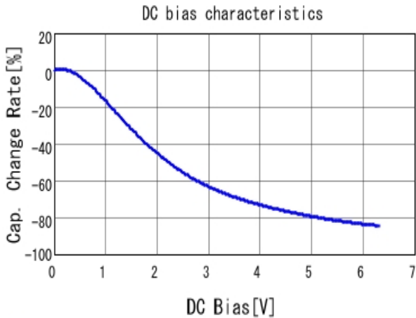
■ GRM155B30J475ME47 C-DC bias capchange, 20.0degC, AC0.
