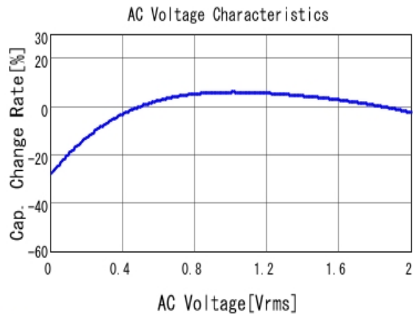
■ GRM155B31A225KE95 C-AC Voltage capchange, DCOV, 20.0d
