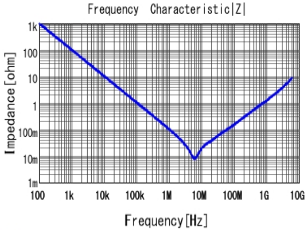
■ GRM155B31A225KE95 |Z| DCOV, 20degC
