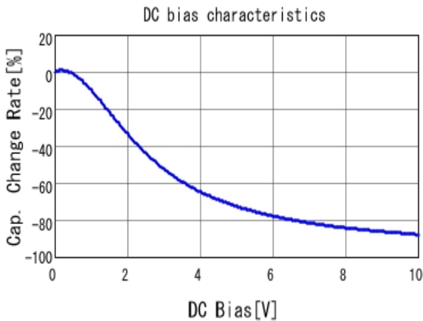
■ GRM155B31A225KE95 C-DC bias capchange, 20.0degC, AC0.
