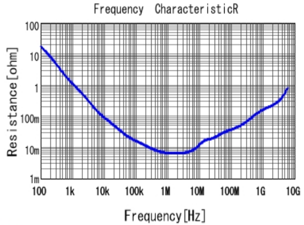
■ GRM155B31A225KE95 R DCOV, 20degC
