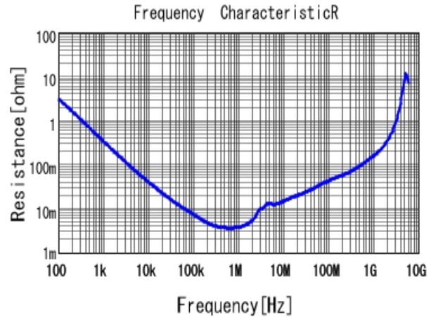
■ GRM319R61C226ME15 R DC0V, 25degC
