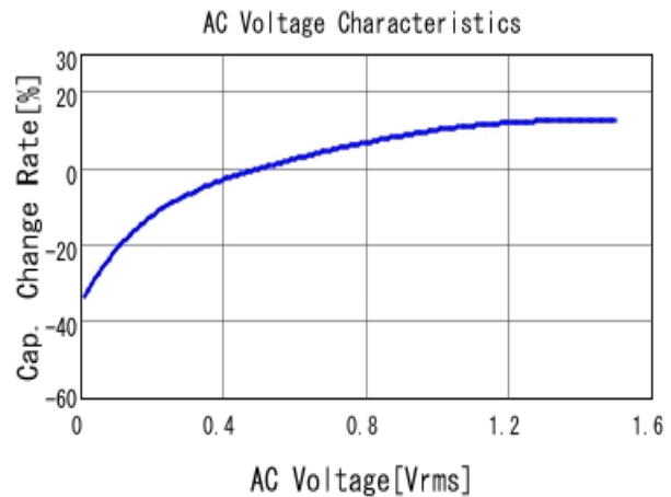
■ GRM319R61C226ME15 C-AC Voltage capchange, DC0V, 25.0d
