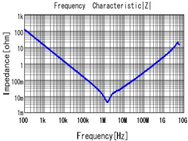
■ GRM319R61C226ME15 |Z| DC0V, 25degC
