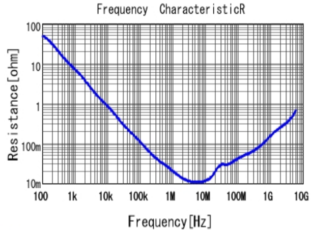
■ GRT155R70J105KE01 R DC0V, 25degC
