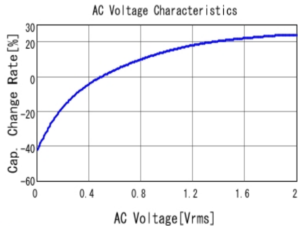
■ GRT155R70J105KE01 C-AC Voltage capchange, DC0V, 25.0d
