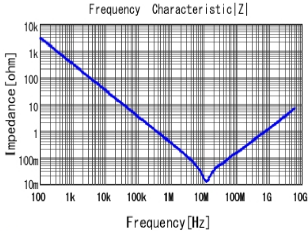
■ GRT155R70J105KE01 |Z| DC0V, 25degC
