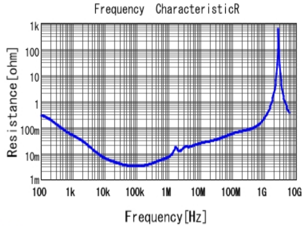
■ KRM55TR71H226MH01 R DCOV, 25degC
