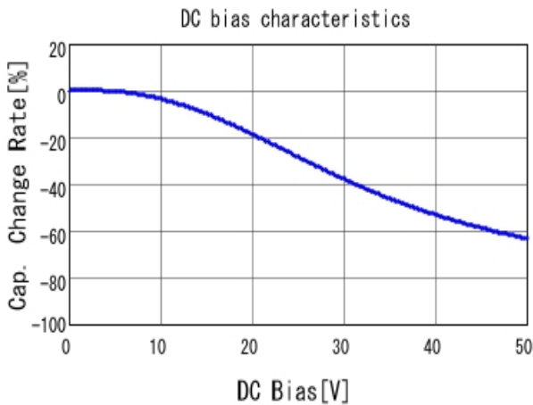
■ KRM55TR71H226MH01 C-DC bias capchange, 25.0degC, AC0.
