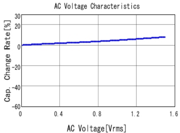
■ KRM55TR71H226MH01 C-AC Voltage capchange, DCOV, 25.0d
