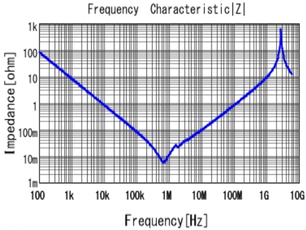
■ KRM55TR71H226MH01 |Z| DCOV, 25degC
