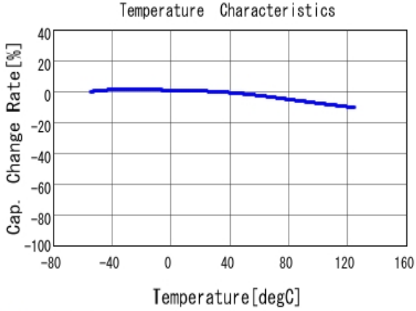
■ KRM55TR71H226MH01 C-Temp. capchange, DCOV, ACO, 5Vrms
