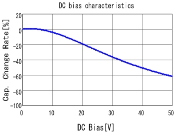
■ KRM55WR71H336MH01 C-DC bias capchange, 25.0degC, AC0.
