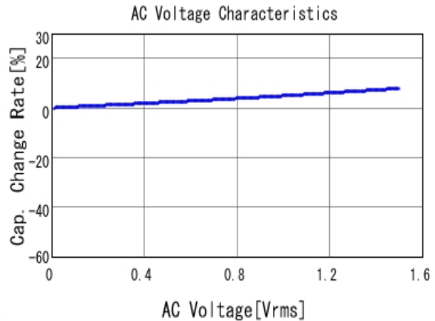
■ KRM55WR71H336MH01 C-AC Voltage capchange, DCOV, 25.0d
