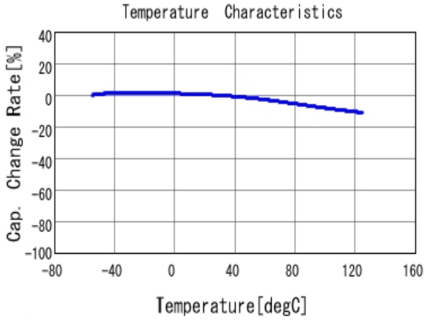
■ KRM55WR71H336MH01 C-Temp. capchange, DCOV, ACO, 5Vrms
