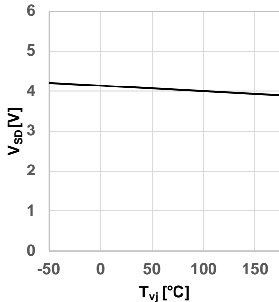
Figure 12 Typical body diode forward voltage as function of junction temperature (V_{SD} = f(T_{vj}), V_{GS} = 0V, I_{SD} = 2A)
