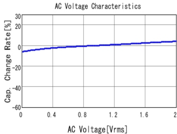
■ GCJ188R71C104KA01 C-AC Voltage capchange, DC0V, 25.0d
